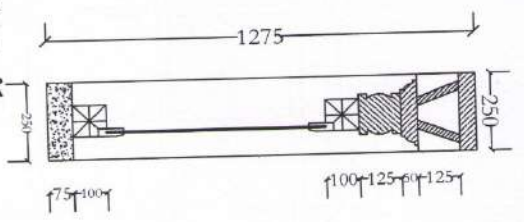
Window W-1 details.
