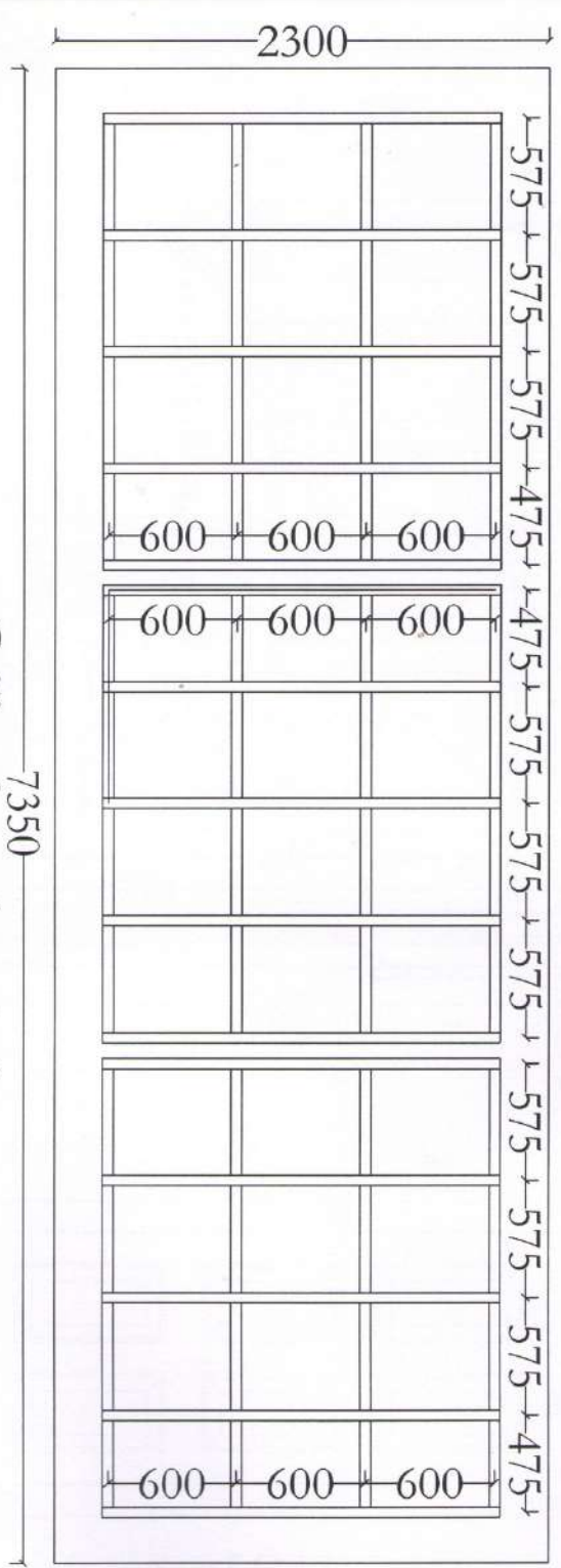
Ceiling frame layout plan.
