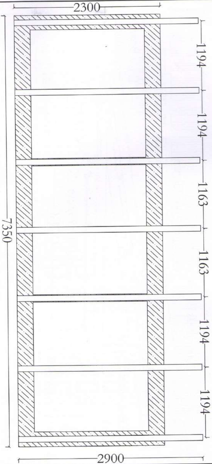
Truss layout plan.
