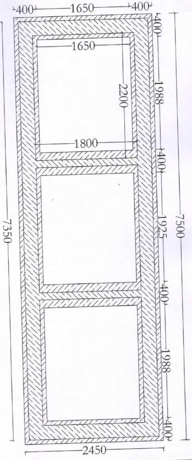
Plan at Floor Level.
